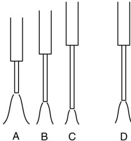
Figure 11. The effect of stickout length on pulsed arc welding. A, B and C show what happens if the welding voltage is kept constant. D is the more ideal case, in which the voltage is allowed to increase somewhat as the stickout increases.
